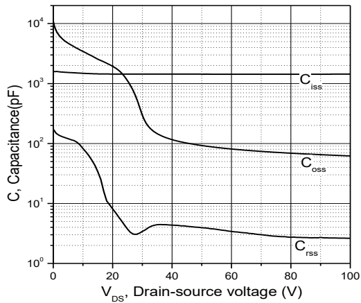
Figure 3. Typ. capacitances
