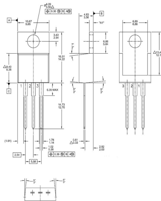
TO - 220
